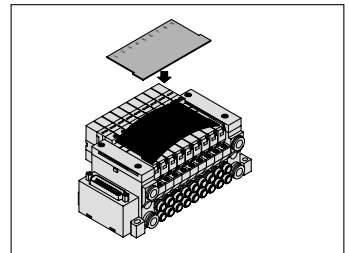
Name plate [-N] VVQ1000-N-Station (1 to Max. stations)
