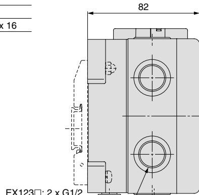
Dust-tight, Water-jet-proof (IP65) SI unit (EX123/124 Integrated-type (output) serial transmission system)
